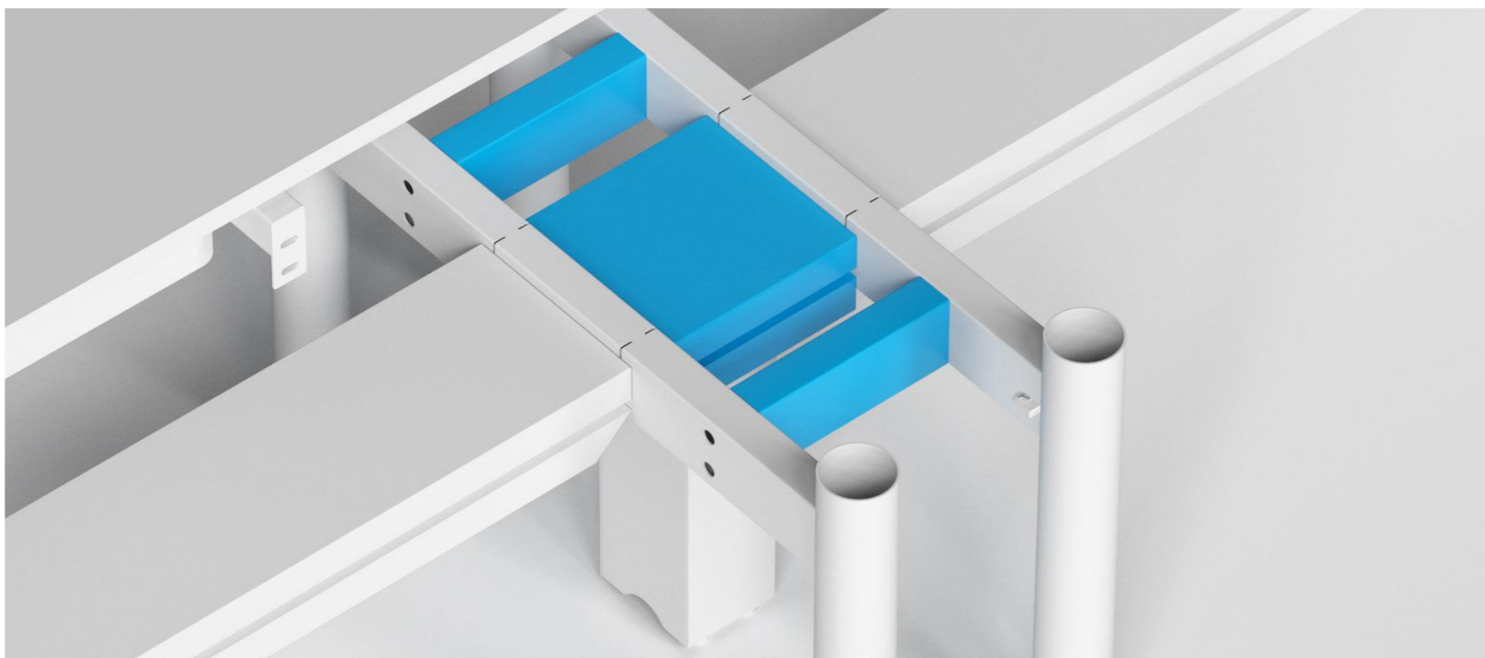
■ Closed cable tray between the back to back workstation for the safety connections.
