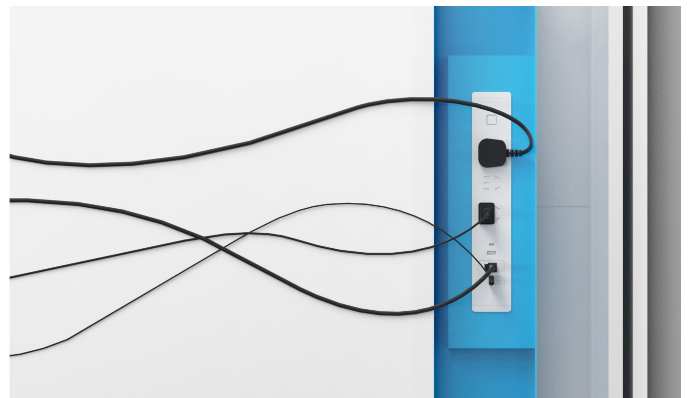
■ The under-desk cable tray is a module way to fixed onto frame instead of traditional fitting way to the table top. It is a dedicated tray for putting integrated power socket and controlling box, in this case, it is easily to install and maintain.
