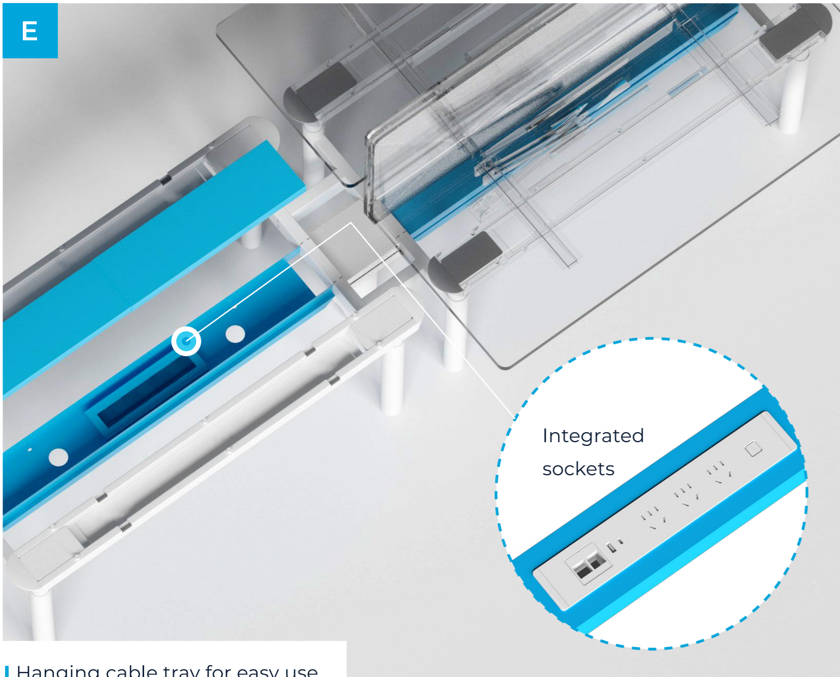
■ With scientific concept, easy installation and less noise when lifting, a bionic design is for a better wire management.
